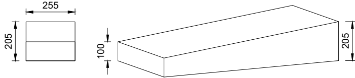
K21 - 255 x 205/100 Conservation Drop Kerb - Right Hand
