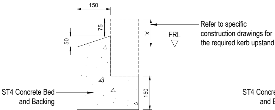
TYPICAL CONCRETE BED AND BACKING TO KERBS
