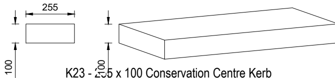
K23 - 255 x 100 Conservation Centre Kerb
