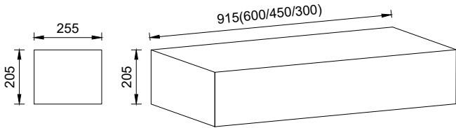
K19 - 255 x 205 Conservation Kerb
