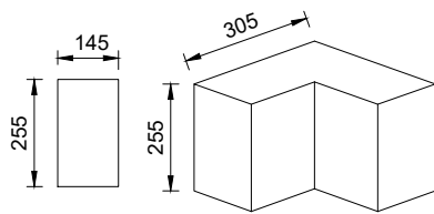
A6 - 145 x 255 Conservation Angle Kerb Internal
