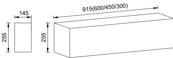
K16 - 145 x 255 Conservation Kerb
