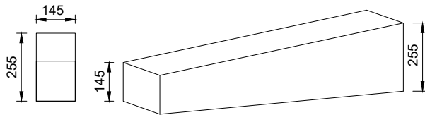
K18 - 145 x 255/145 Conservation Drop Kerb - Right Hand
