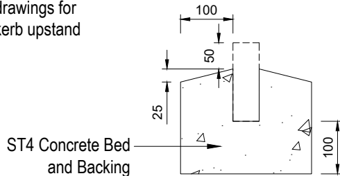
TYPICAL CONCRETE BED AND BACKING TO EDGINGS
