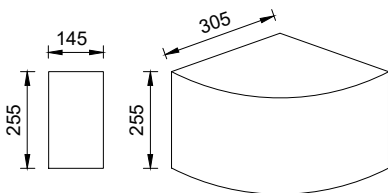
Q5 - 305 x 255 Half Battered Quadrant Kerb
