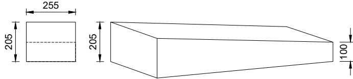
K20 - 255 x 205/100 Conservation Drop Kerb - Left Hand
