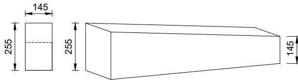
K17 - 145 x 255/145 Conservation Drop Kerb - Left Hand
