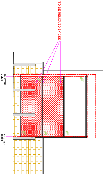
EXISTING ELEVATION
