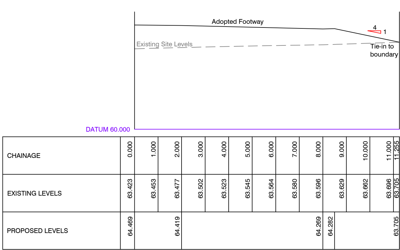
ROAD 2A SECTION B-B
