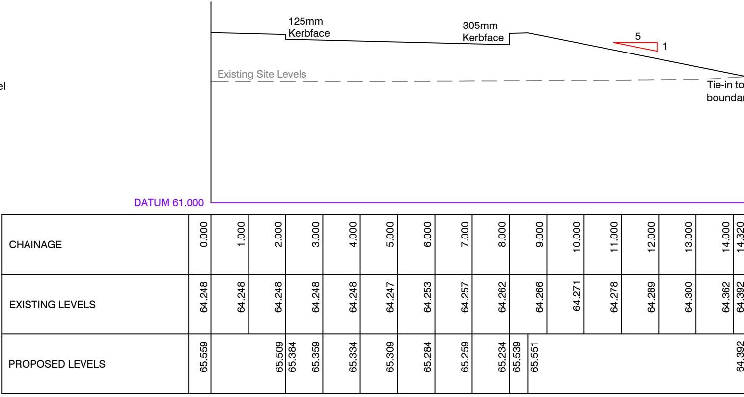
ROAD 2A SECTION A-A
