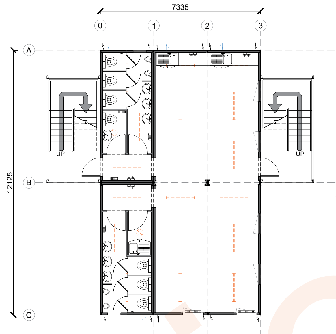
Ground Floor Plan, 1:100@A2
