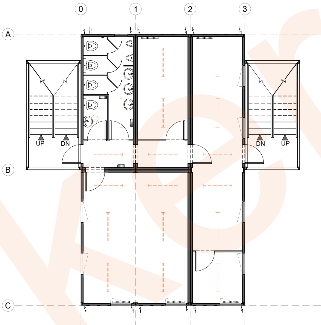
First Floor Plan, 1:100@A2
