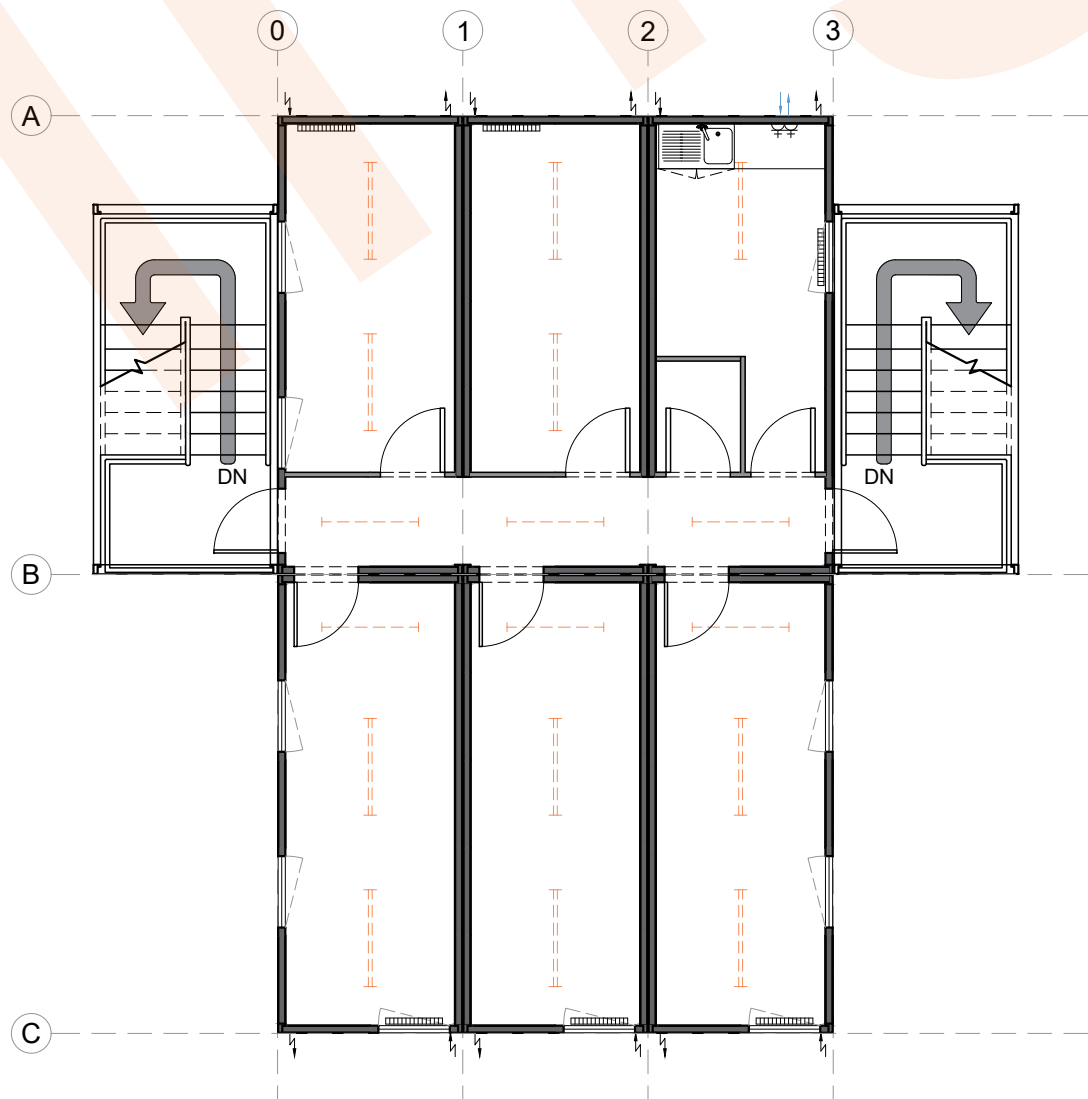
Second Floor Plan, 1:100@A2
