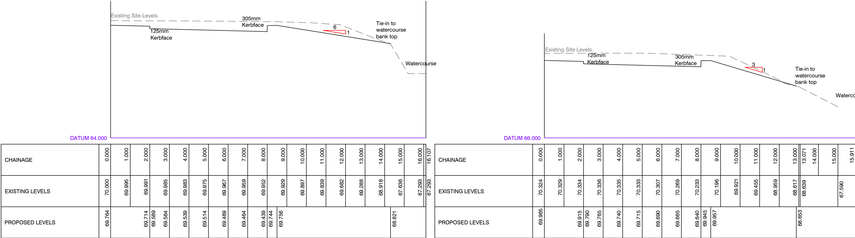
ROAD 7A SECTION I-I
