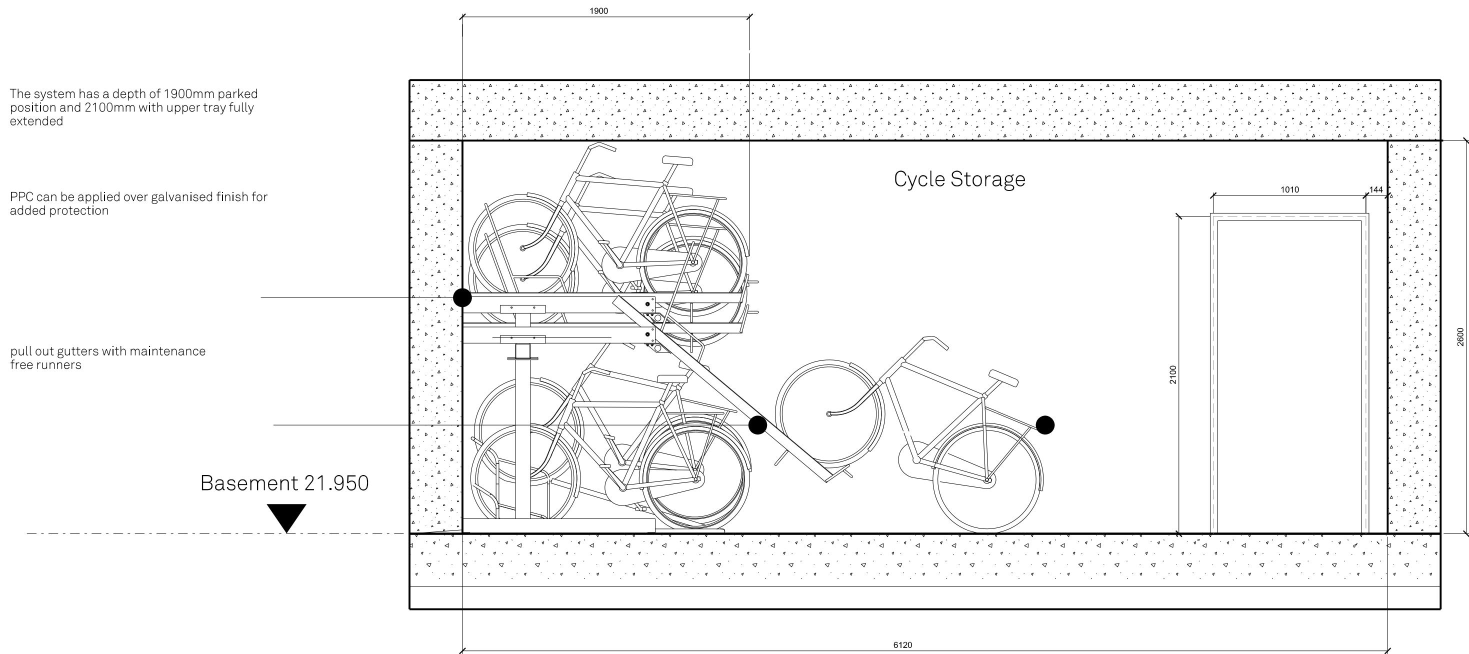
SECTION B
