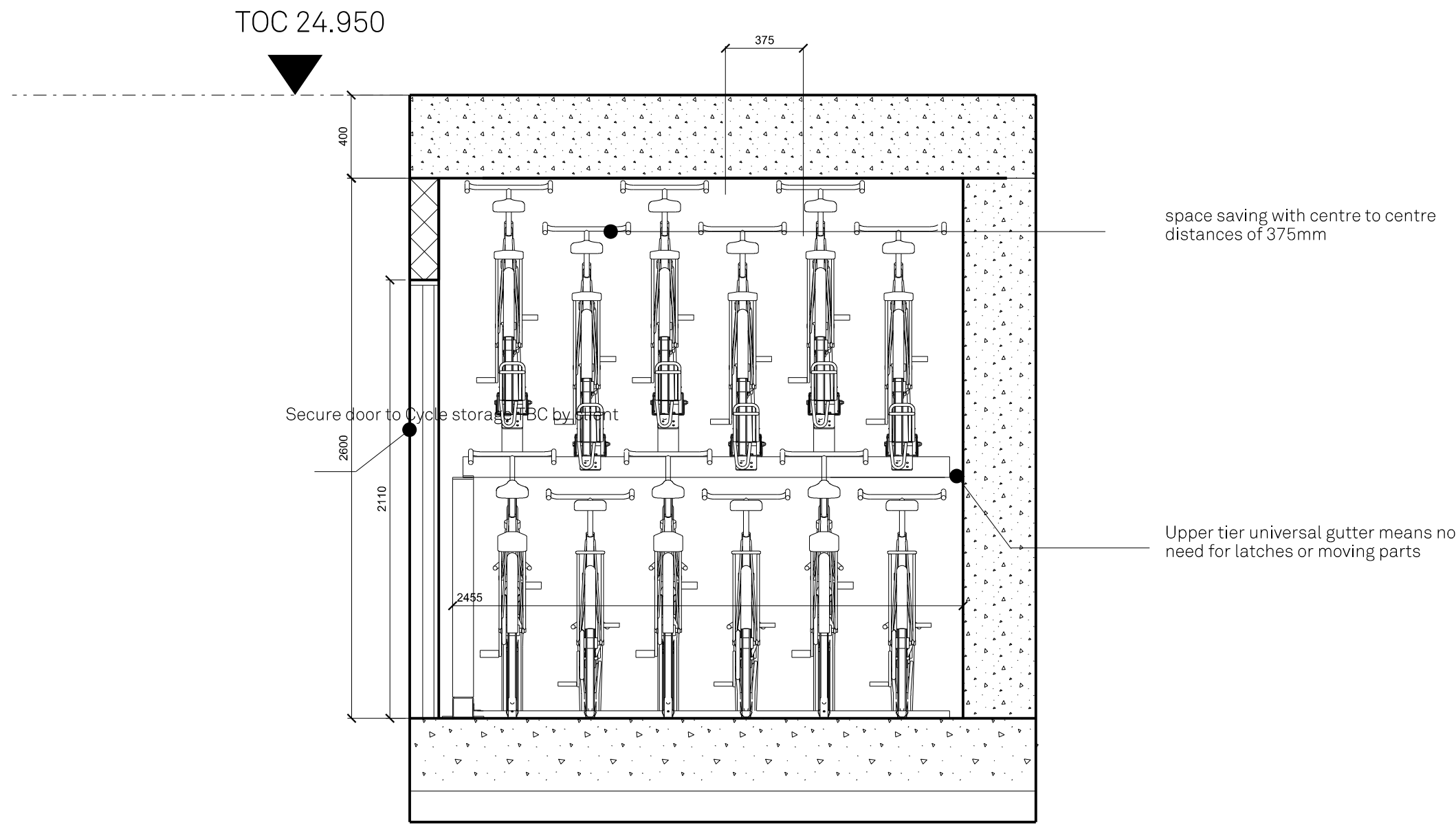
SECTION A
