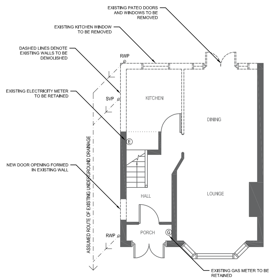
EXISTING GROUND FLOOR LAYOUT
