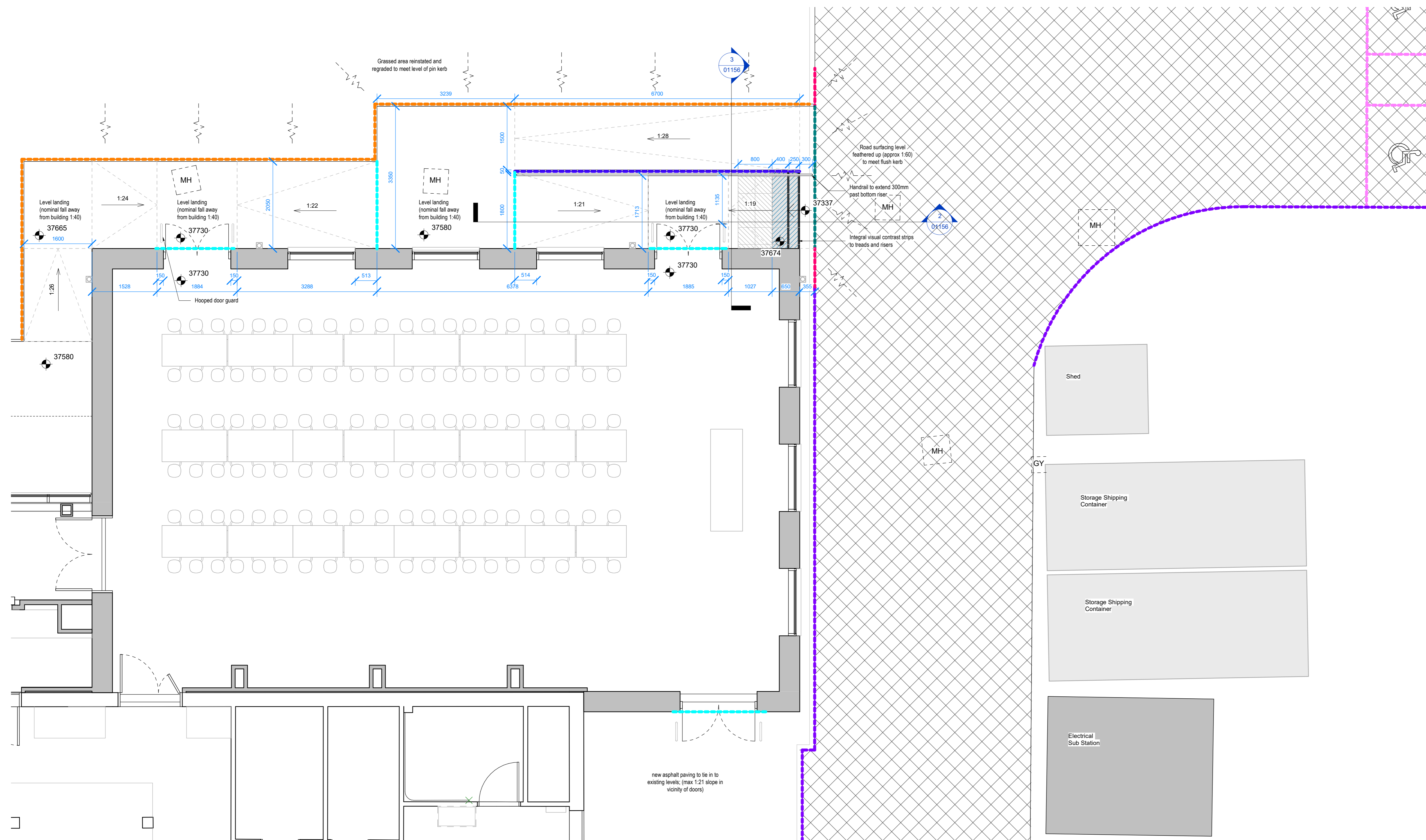
Phase 1 - Proposed External Level Access Works Plan 1 : 50
