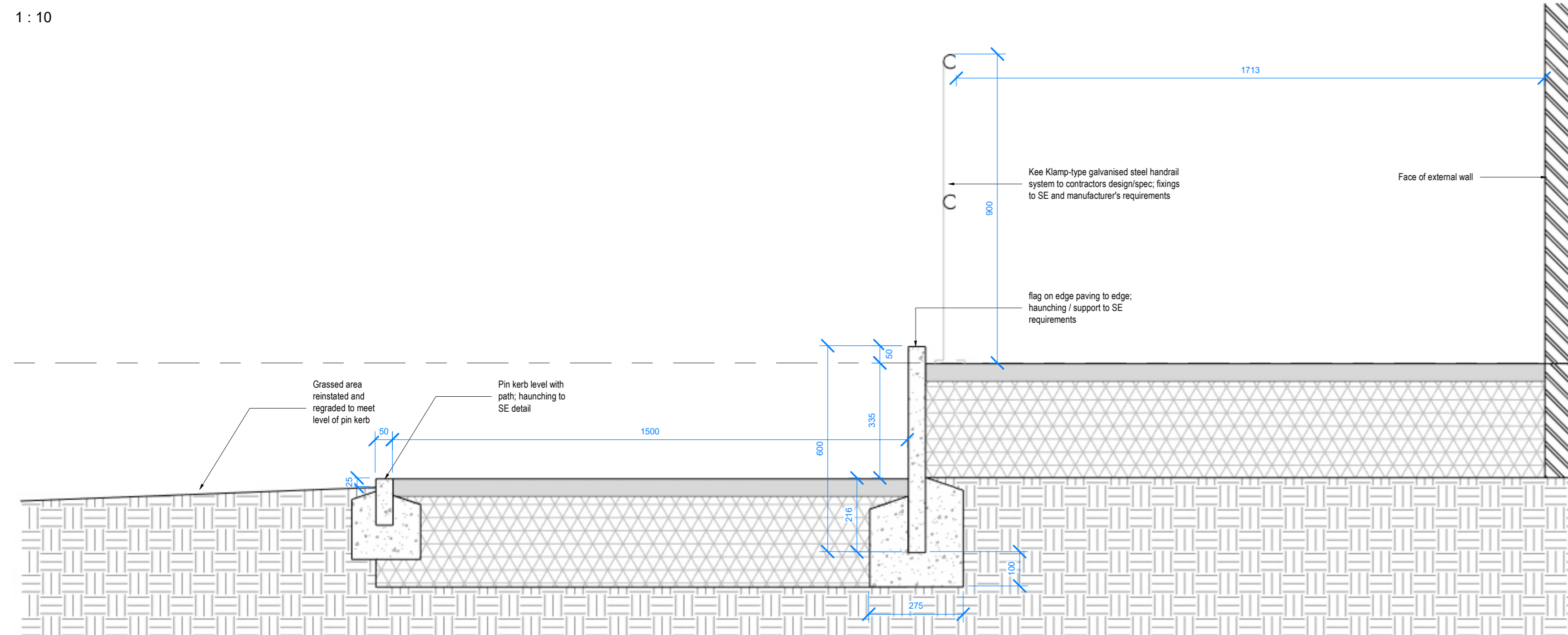
3. Phase 1 - Sloped access cross-section 1 : 10
