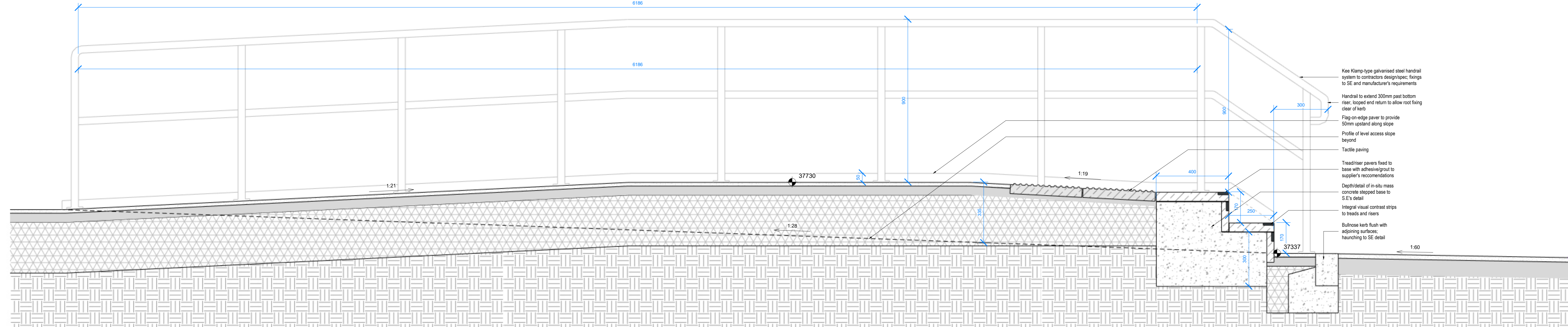
2. Phase 1 - Stepped access section 1 : 10
