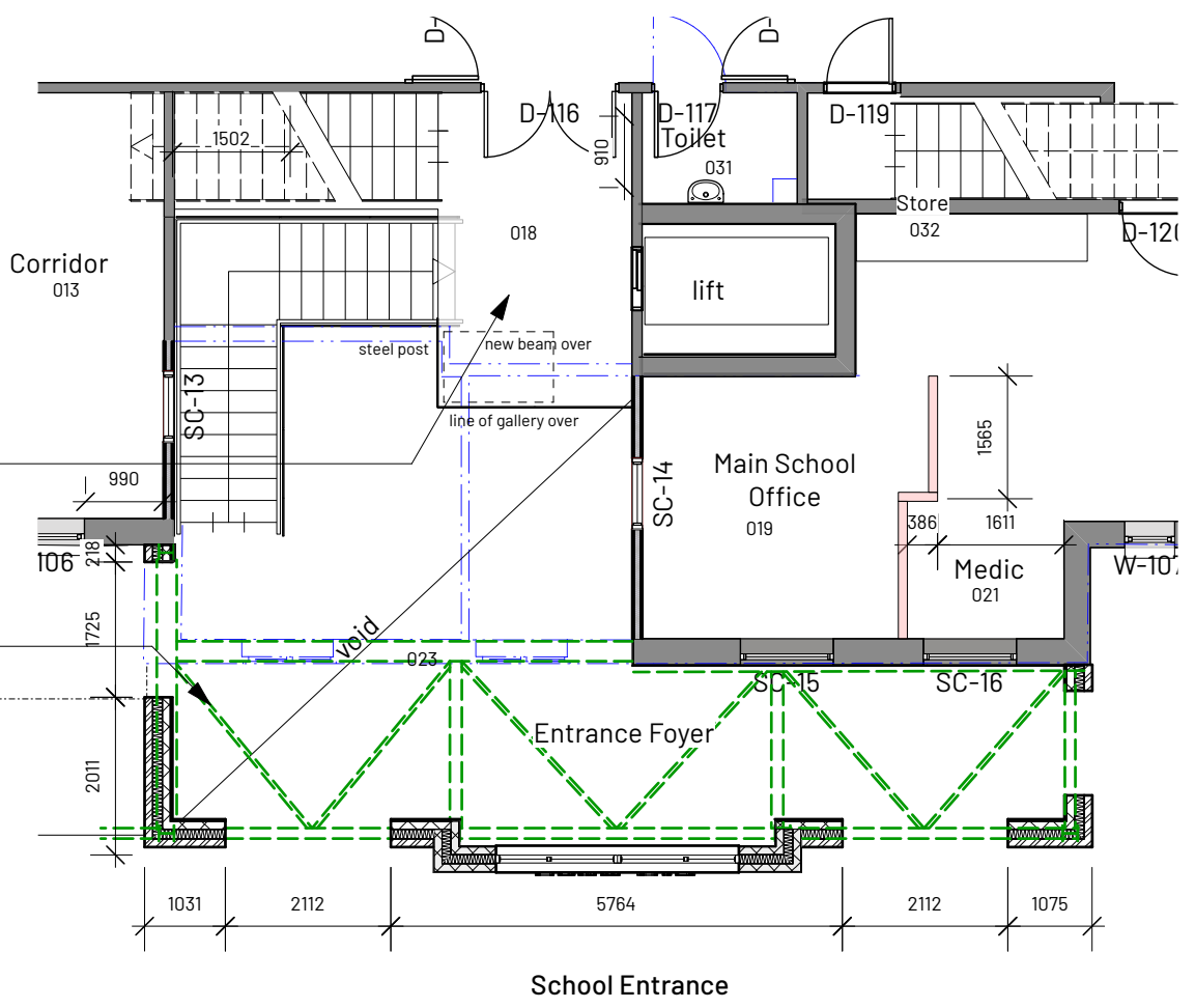
2 Proposed First Floor Entrance Plan Scale: 1:100
